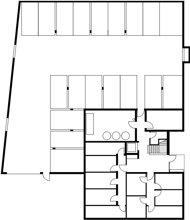
Piano terreno
