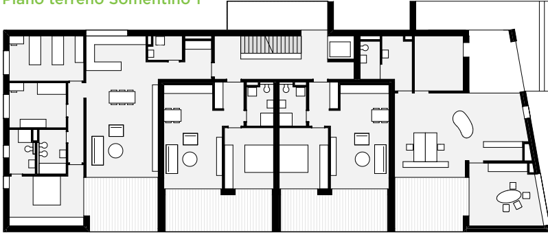
Piano terreno Somentino 1
